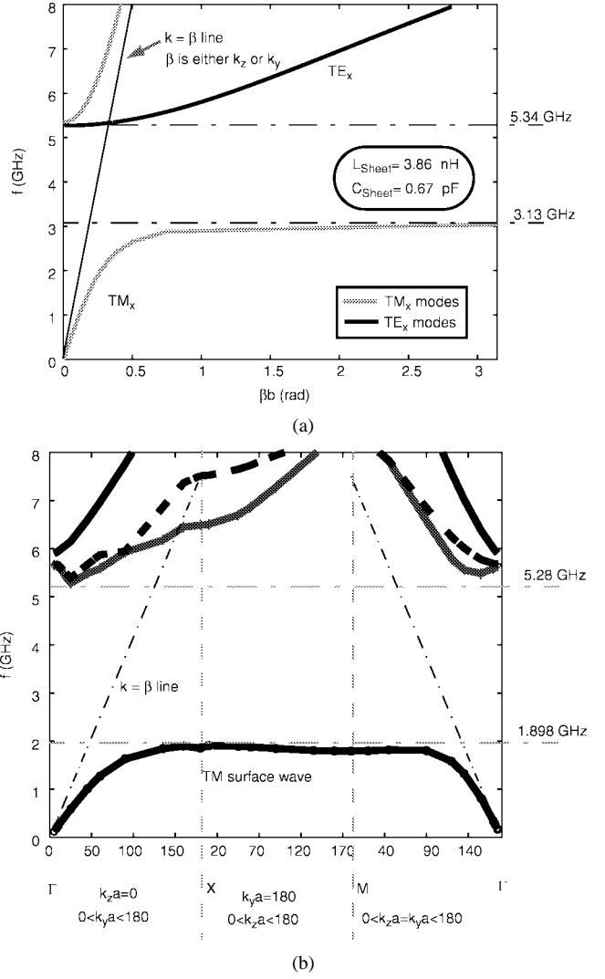
Fig. 7. Dispersion diagrams of the two-layer structure shown in Fig. 3(b). (a) TRM solutions. (b) FEM simulations.
