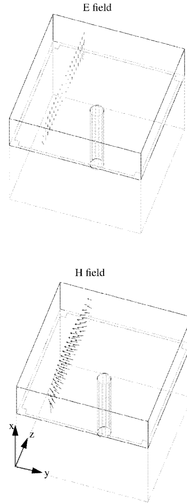
Fig. 9. E - and H -field profiles in the \Gamma-X section of the dispersion diagram at k_y a = 135^\circ for the second mode, which appears to be a hybrid mode.
