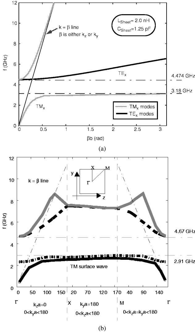
Fig. 6. Dispersion diagrams of the three-layer structure shown in Fig. 3(a). (a) TRM solutions. (b) FEM simulations.
