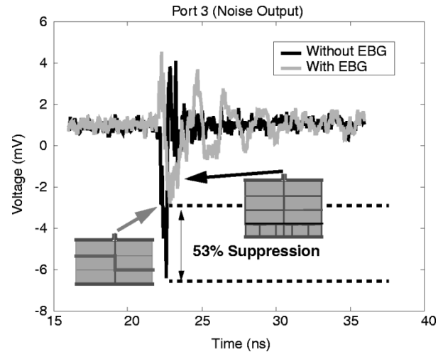
Fig. 17. Probed noise voltages from the TDR measurements of two stripline-via structures; one has the same partial ground configuration as the test-bed in Fig. 13(a) (but with the two-layer EBG surface instead of the three-layer one) and the other is the structure of Fig. 13(b).
