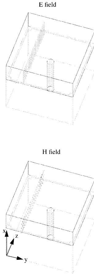
Fig. 8. E - and H -field profiles in the \Gamma-X section of the dispersion diagram at k_y a = 135^\circ for the first mode, which has a TM_x pattern.
